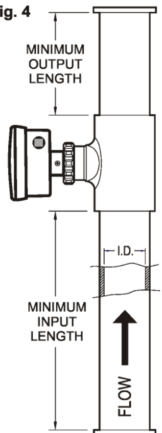
Vertical Mount
